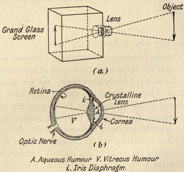
FIG. 4.—Comparison of Eye with Photo Camera.
