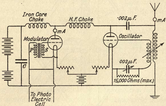
FIG. 93.—Transmitting Radio-circuit.
