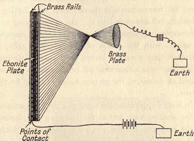
FIG. 14.—Senlecq's Apparatus.
