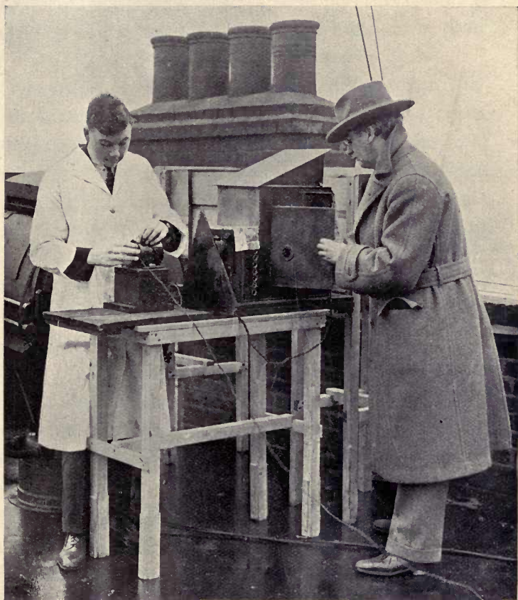
FIG. 96.—Mr. Baird testing the Fog-penetrating Power of his "Noctovisor."
