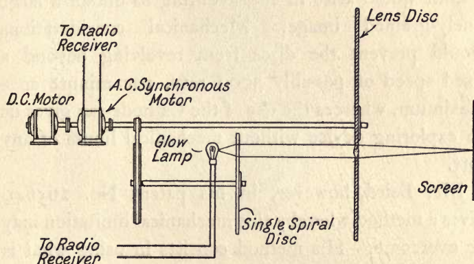
FIG. 83.—Diagrammatic Sketch of Receiving Apparatus.
