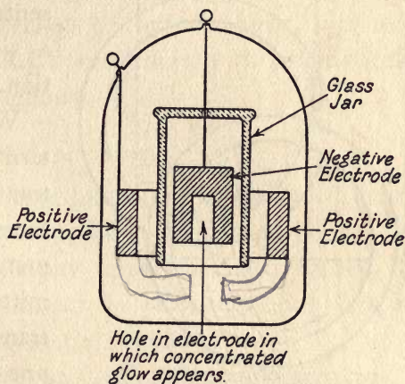
FIG. 60.—The Moore Lamp.
