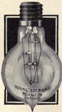
FIG. 20.—Pointolite Lamp.
