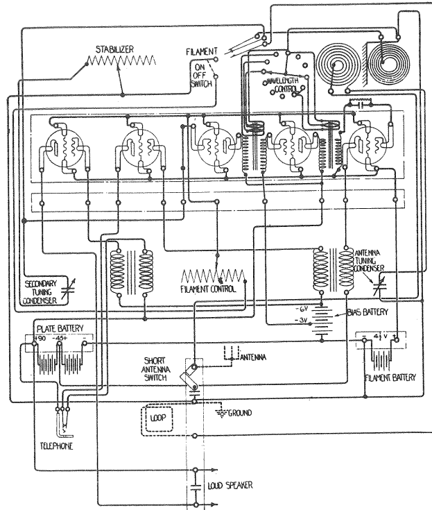
WIRING DIAGRAM
