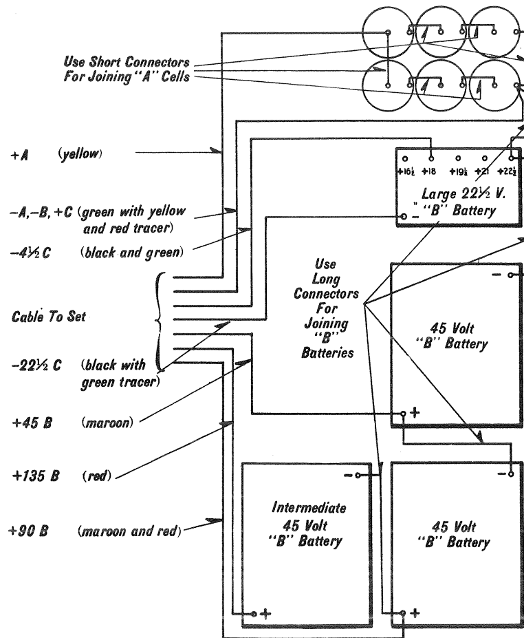
RADIOLA 20.- BATTERY CONNECTIONS.
