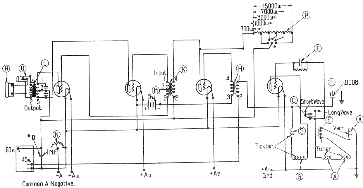
Diagrammatic Connection of Dry Cells
