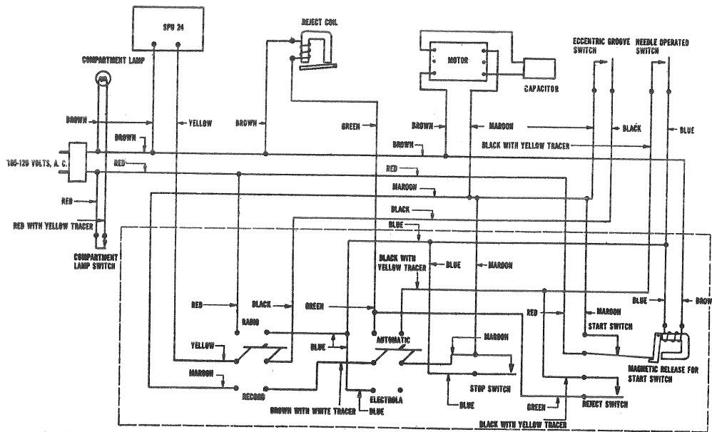
A. C. Power Wiring Diagram Automatic Electrola No. 10-69 Below Serial No. 3501
