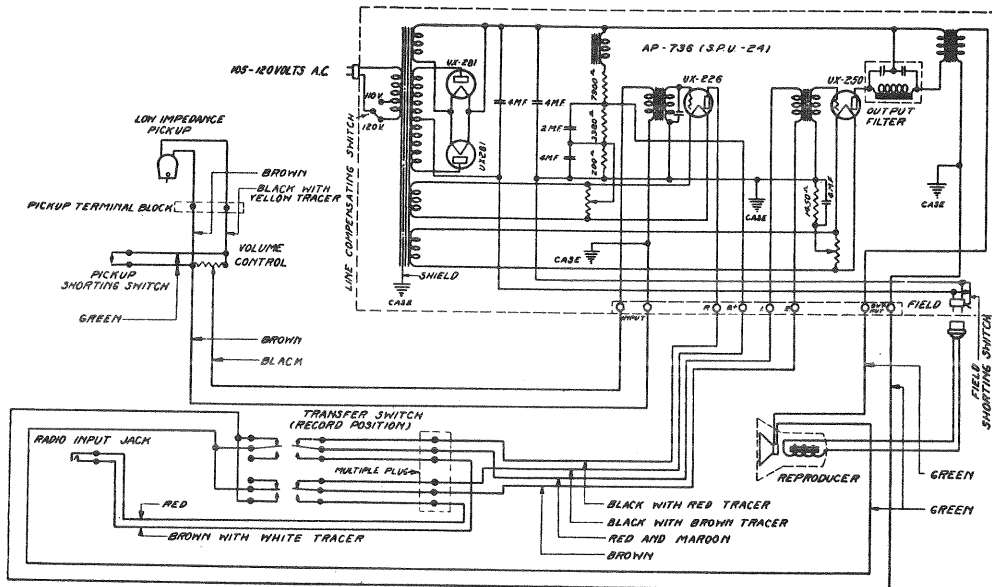
Schematic Wiring Diagram Automatic Electrola 10-69 above serial No. 2600
