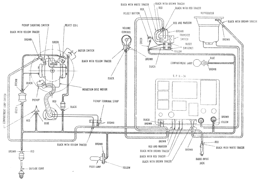
-Wiring Diagram for Automatic Electrola No. 10-70 Showing connections between terminals of the various units.
