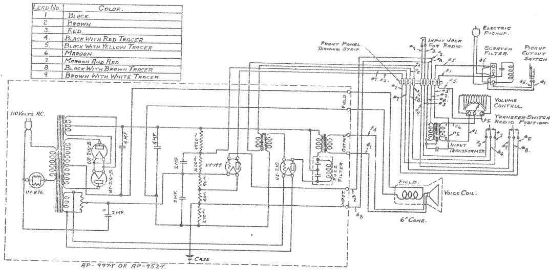
Wiring Diagram—Electrola 10-70
