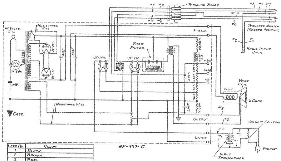
Wiring Diagram Electrola 12-15
