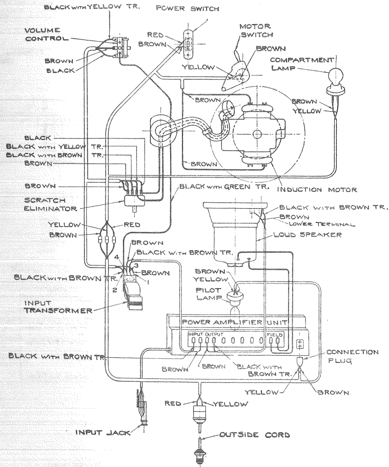
-Schematic Wiring Diagram of Electrola 12-25 Showing connections between terminals of the various units.
