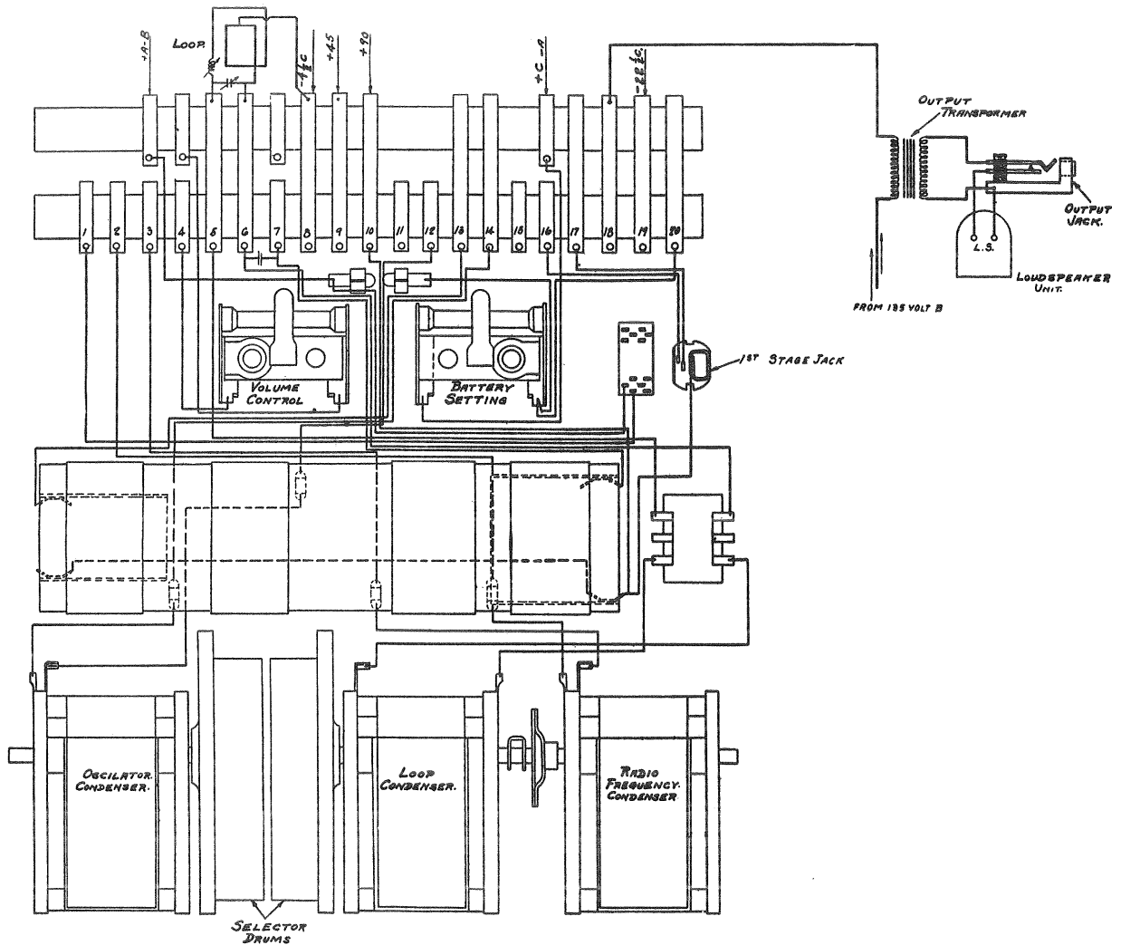
Panel Assembly Diagram for Borgia I
