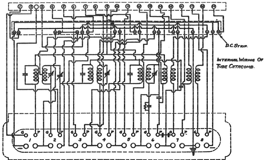
Radiola 28 Catacomb Continuity Diagram for Model 9-3
