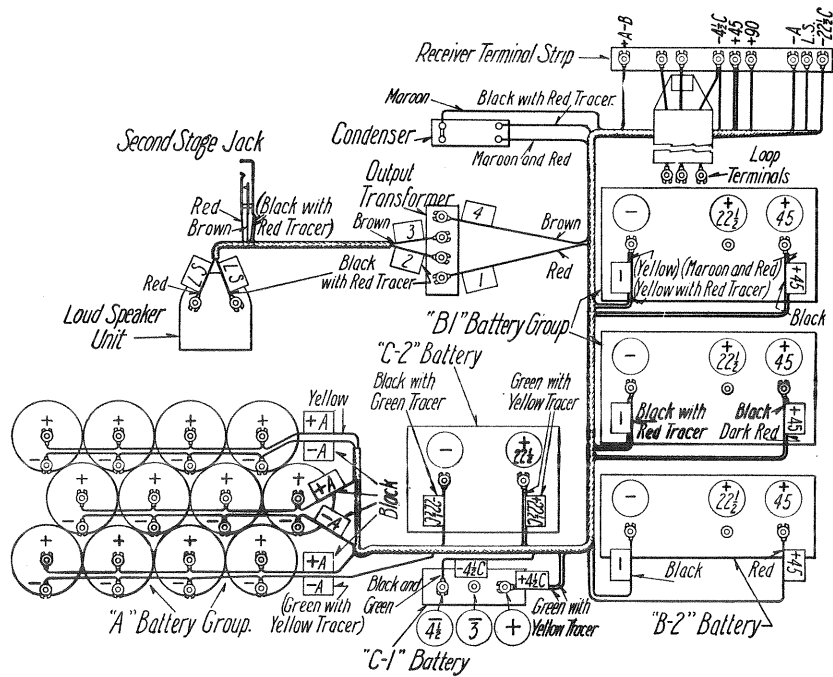
Battery Connection Diagram
