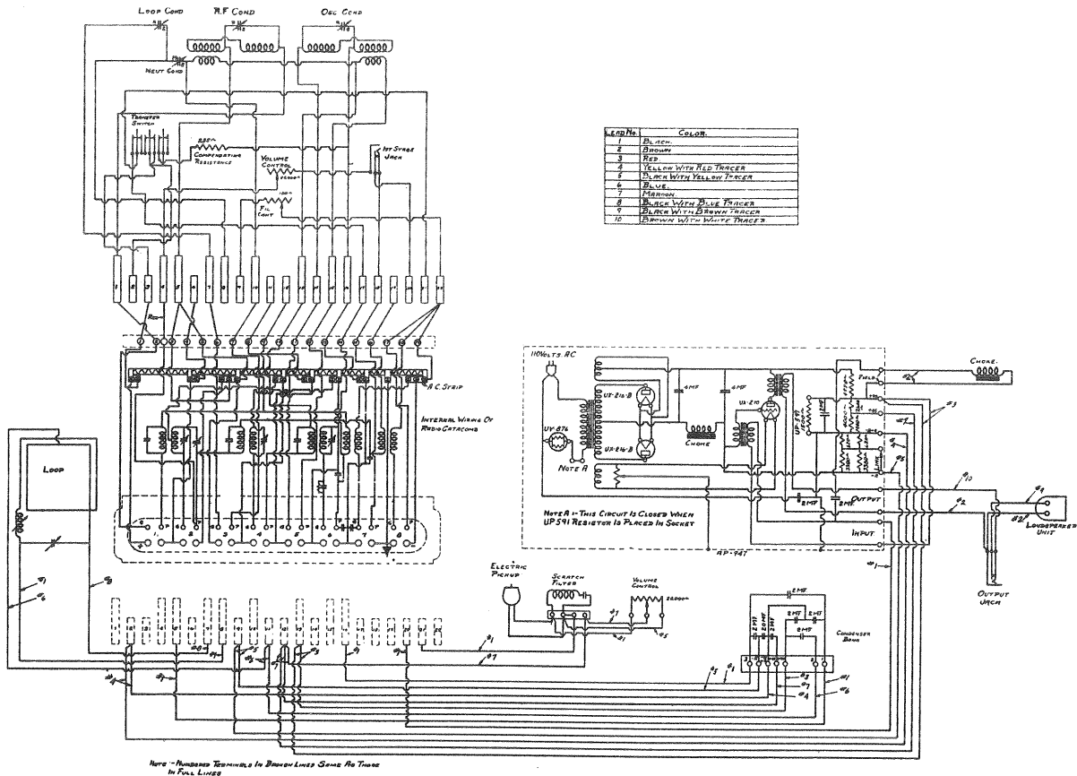
Wiring Diagram for Electrola 9-40
