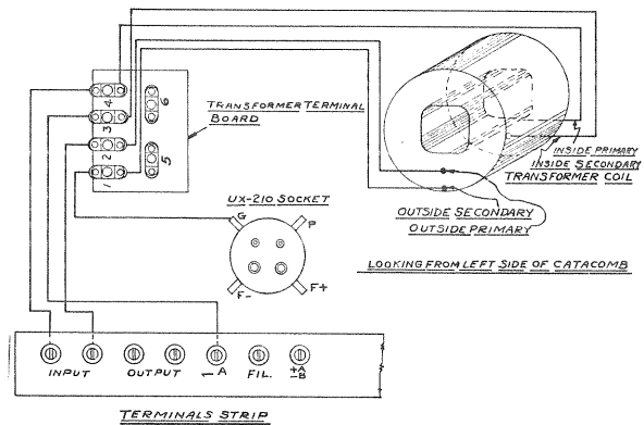
9-40 Input Transformer Wiring
