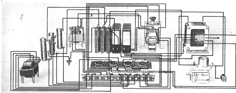
Parts and Wiring of Power-Amplifier Units
