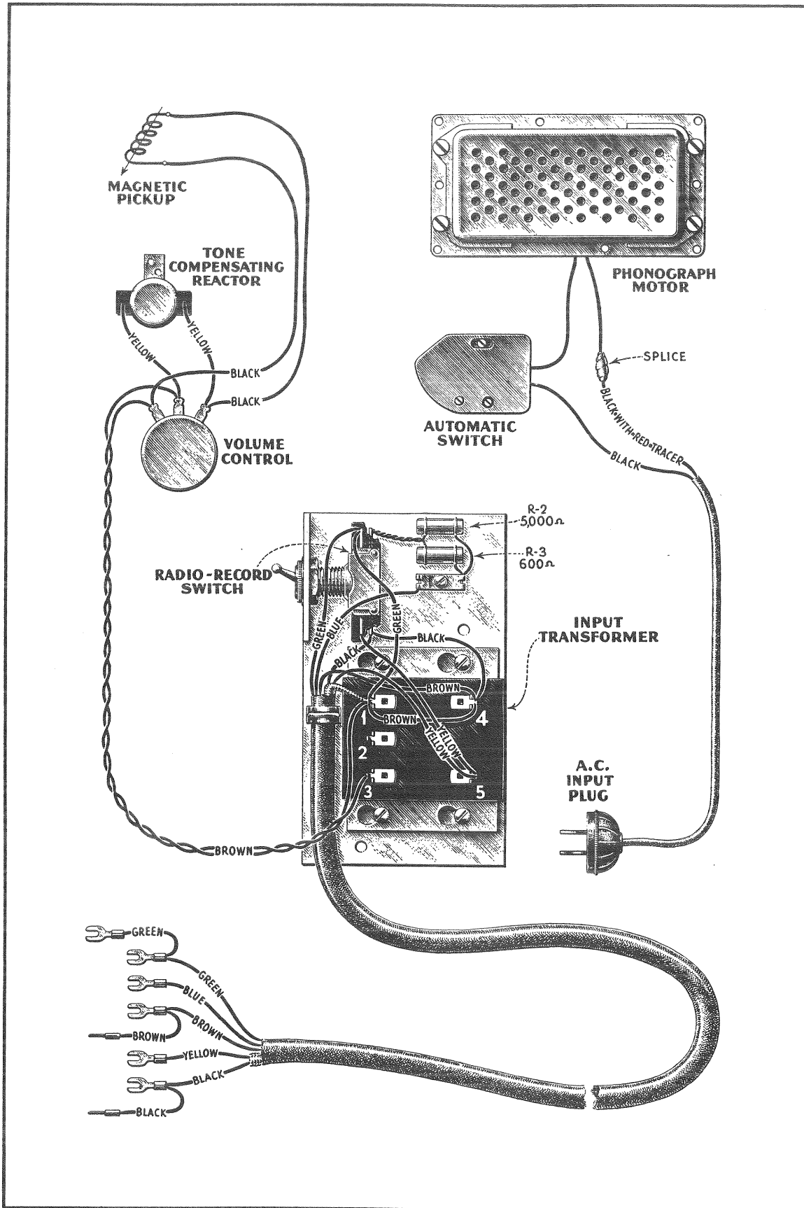
Figure 1—Assembly Wiring
