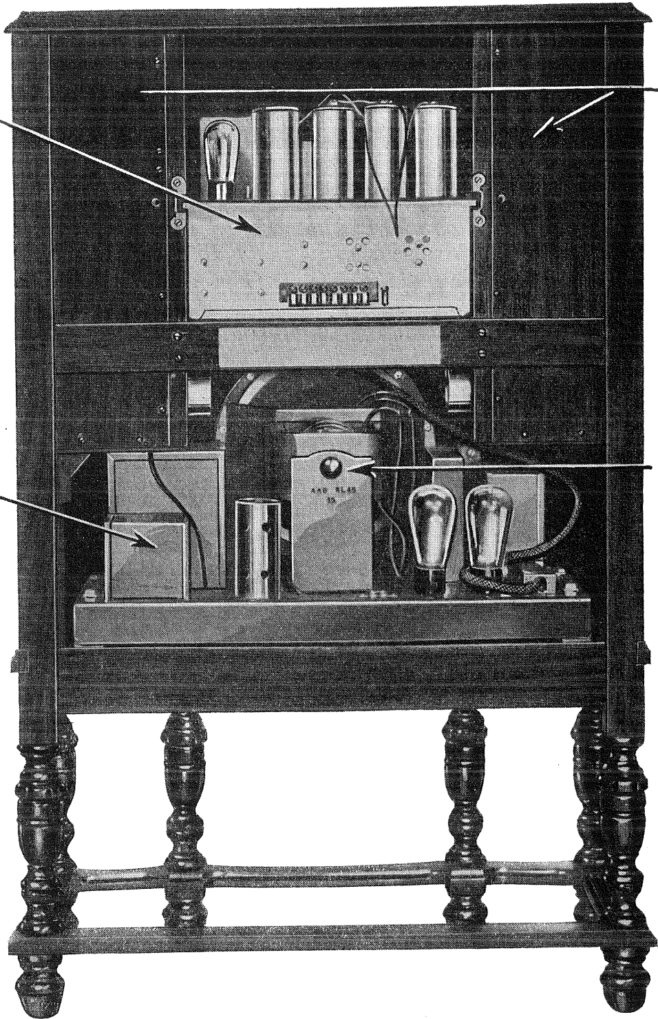
Figure 1—Rear Interior View of R-78
