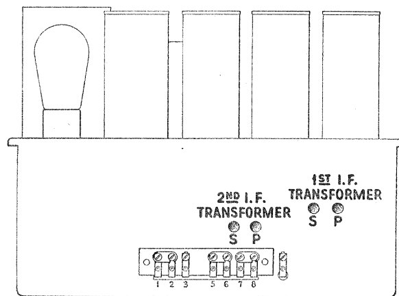
Figure 7—Location of I. F. Tuning Capacitors
