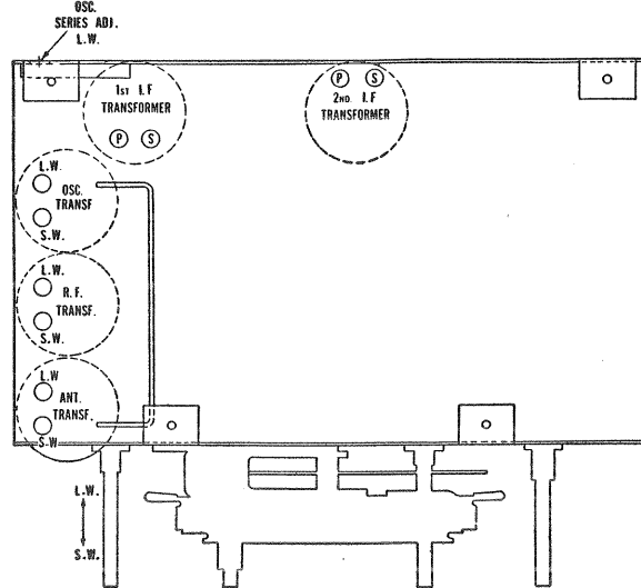
Figure E—Location of Line-Up Capacitors
