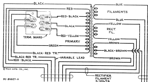
Figure 8—Universal Transformer
