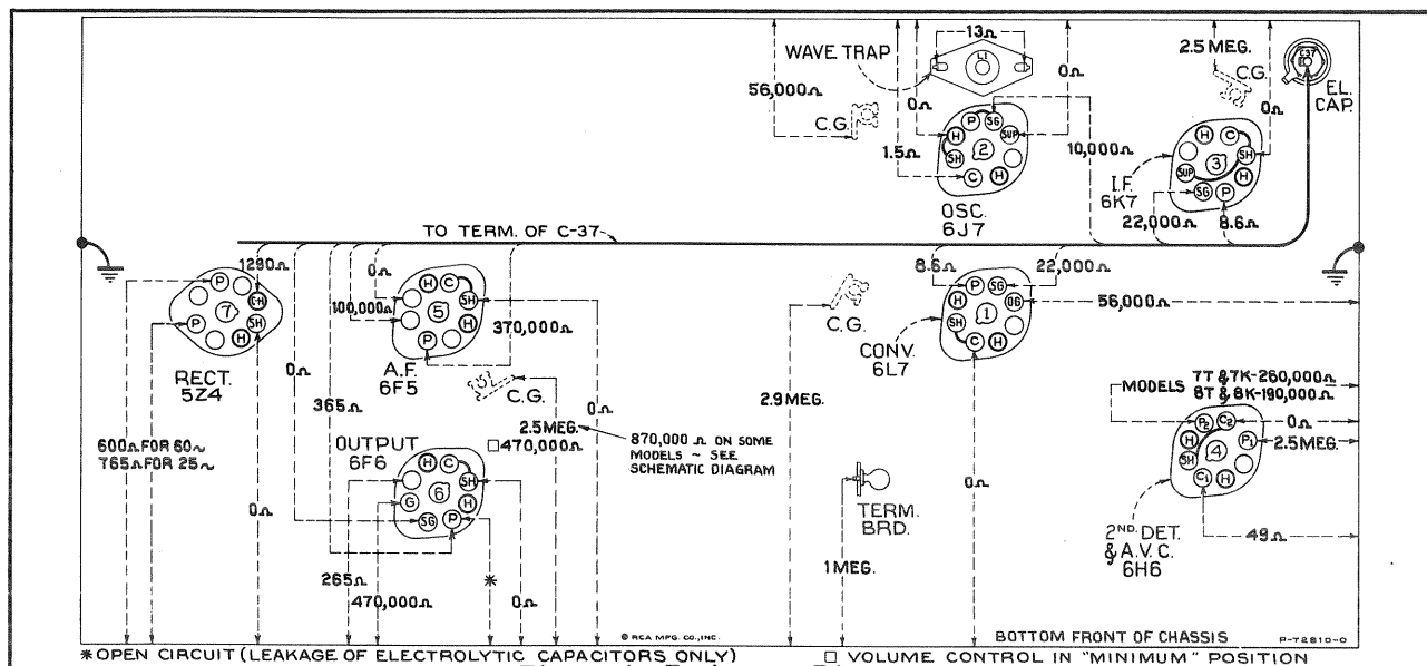
Figure 6—Resistance Diagram
