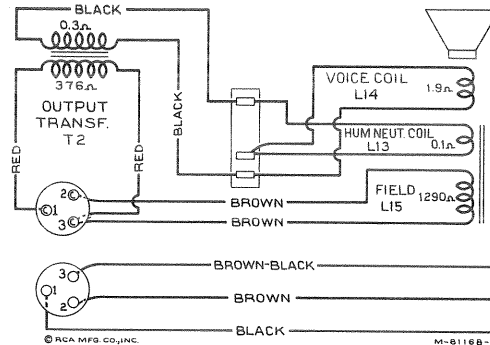
Figure 5—Loudspeaker Wiring
