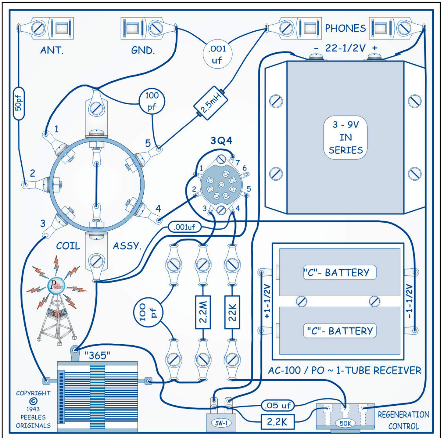
Chassis Part's Placement, Template, Full-Size.
