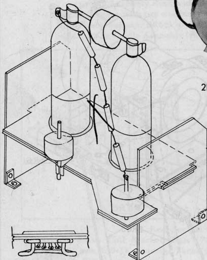
Corona Ring Detail
