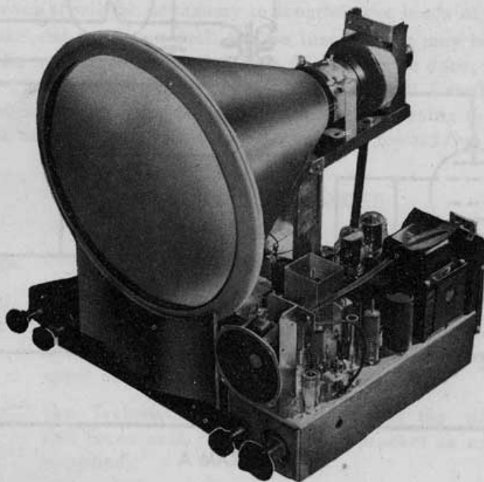
Tech-Master 630-TK Chassis With 16AP4 Kinescope Using Tech-Master Universal Adjustable Brackets 16AP4 is shown with plastic mounting ring and sleeve.
