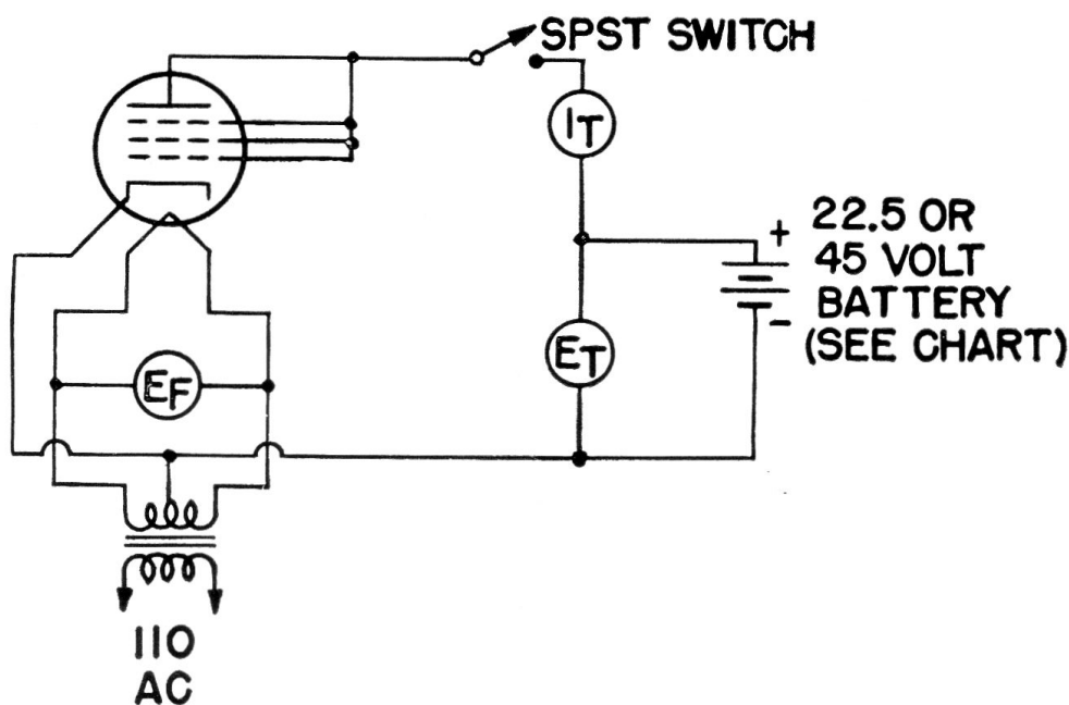
Fig. 3. Circuit diagram for limited peak emission test.
