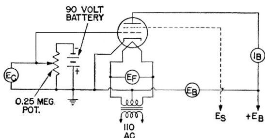
Fig. 1. Circuit diagram for static characteristic test set.
