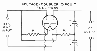
R = HEATERS OF OTHER TUBES IN SERIES WITH VOLTAGE-DROPPING RESISTOR R_L = PROTECTIVE RESISTOR
