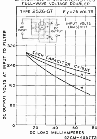
OPERATION CHARACTERISTICS
