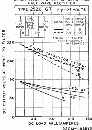
OPERATION CHARACTERISTICS
