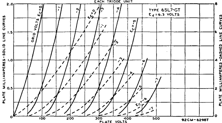
AVERAGE PLATE CHARACTERISTICS EACH TRIODE UNIT
