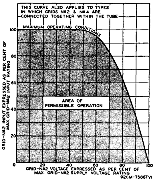
Fig. 95—Grid-No.2 input rating curve.
