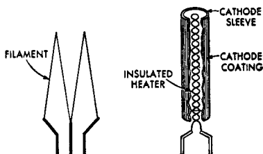
Fig. 1—Filament or directly heated cathode.
