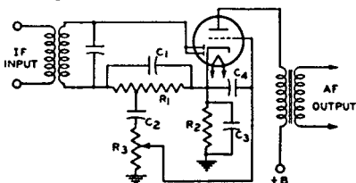
Fig. 51—Typical diode-detector circuit using a twin diode—triode tube.
