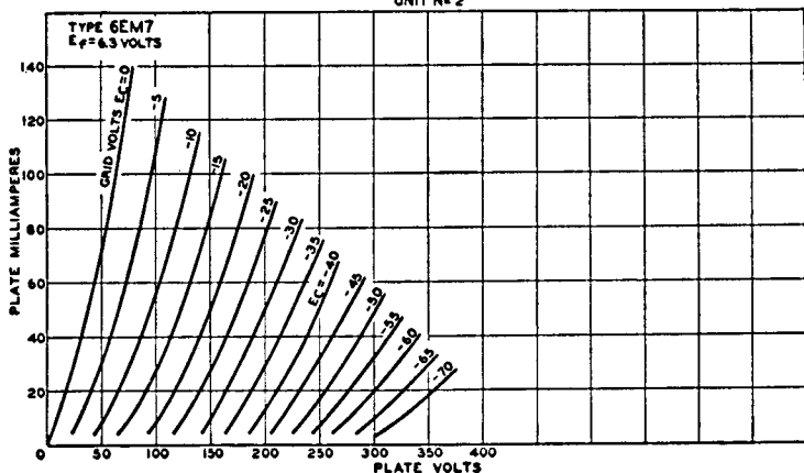
AVERAGE PLATE CHARACTERISTICS UNIT NR 2
