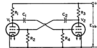
Fig. 69—Basic multivibrator circuit of the free-running type.
