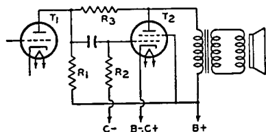
Fig. 29—Resistance-coupled stages using feedback resistor.
