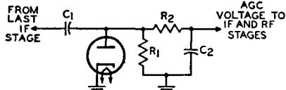
Fig. 62—Automatic-gain control (agc) circuit.
