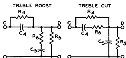
Fig. 39—Simplified representations of treble-control circuit at extreme ends of potentiometer.
