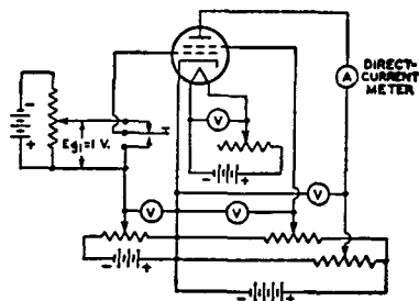
Fig. 101—Fundamental circuit of a transconductance tester using the "grid-shift" method.
