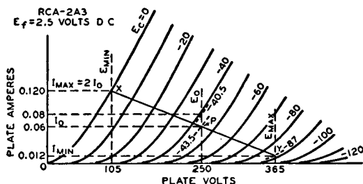
Fig. 20—Graphic calculations for class A amplifier using the 2A3 power triode.
