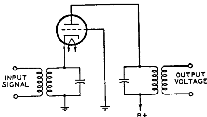
Fig. 26—Cathode-drive circuit.
