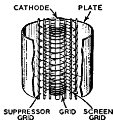
Fig. 16—Structure of remote-cutoff grid.
