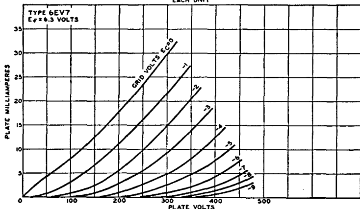
AVERAGE PLATE CHARACTERISTICS EACH UNIT
