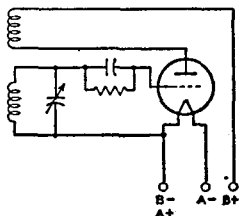
Fig. 67—Tuned-grid triode oscillator circuit using filament-type tube.
